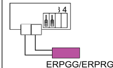
Figure 3 Switch setting and wiring for internal setpoint and external sensor.
